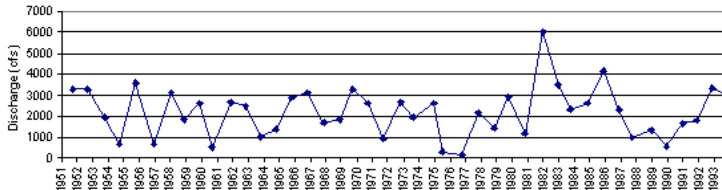
Peak Discharge Corte Madera Creek at Ross, CA USGS 11460000
